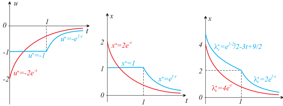
In red: the optimal tern of the problem (3.108), in the case r = 2, a = 3, b = 1, x_0 = 2 . In blue: the optimal tern of the problem (3.114).
