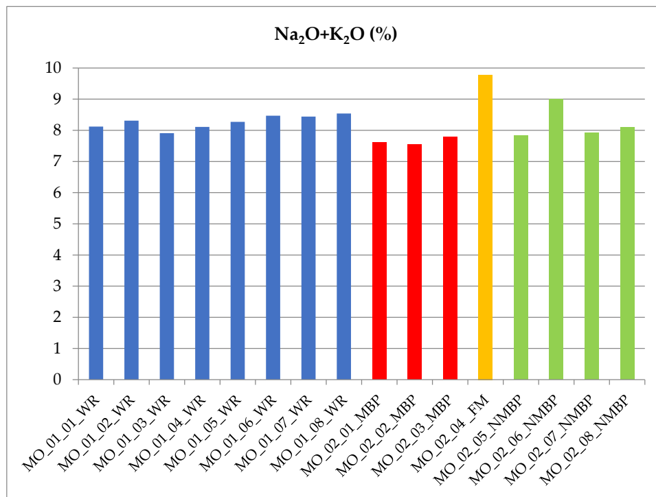
Figure 9. Concentration of alkalis in the Montorfano pilot (all samples; values in wt %). blue: WR; red: treatment plant, magnetic fraction (MBP); green: treatment plant, nonmagnetic fraction (NMBP), orange: feeding material (FM).
