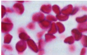
Fetal and adult type globin genes
