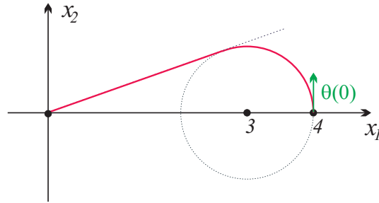
The initial data for the car is (x_1(0), x_2(0), \theta_1(0)) = (4, 0, \pi/2) ; the final position is (x_1(T^*), x_2(T^*)) = (0, 0) with \theta_1(T^*) free.
